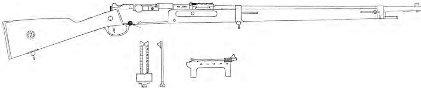
A sketch of a French Level Model 1886 rifle as used by the French Palma team in 1903.
